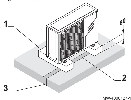
Fig.29 Installation au sol
