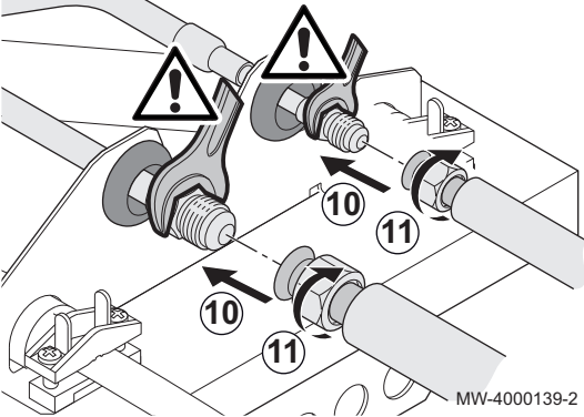
Fig.38 Raccordement des tuyaux
