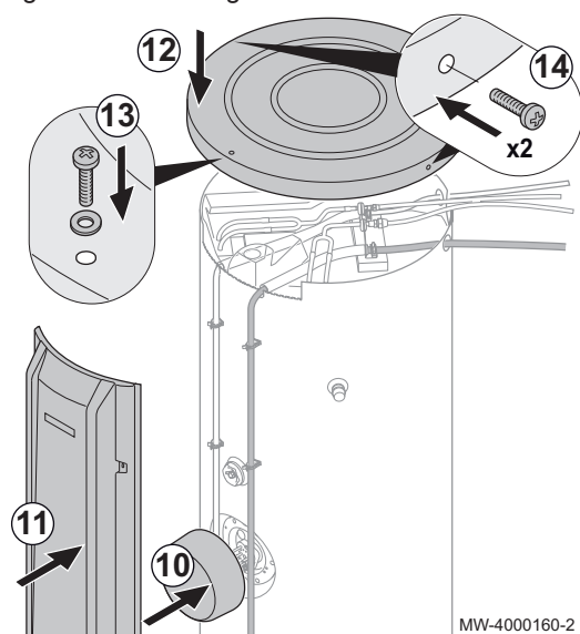
Fig.58 Remontage
