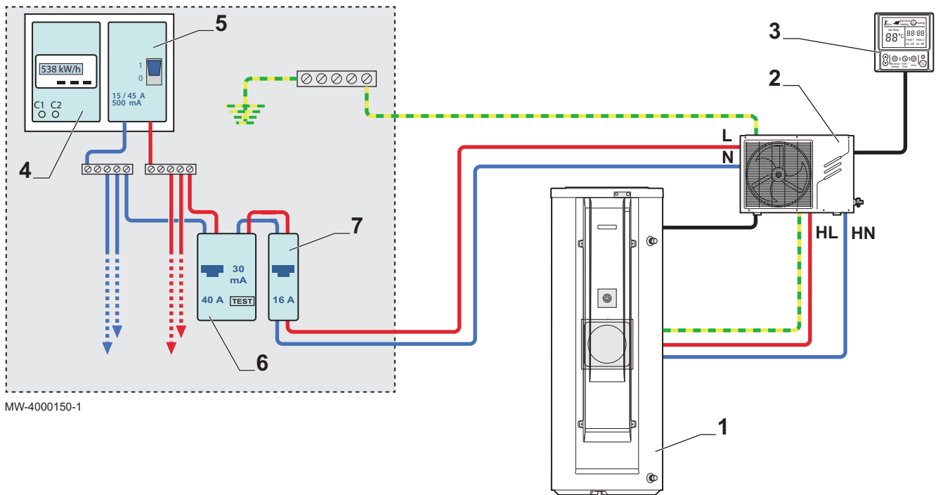
Fig.49 Branchement direct
